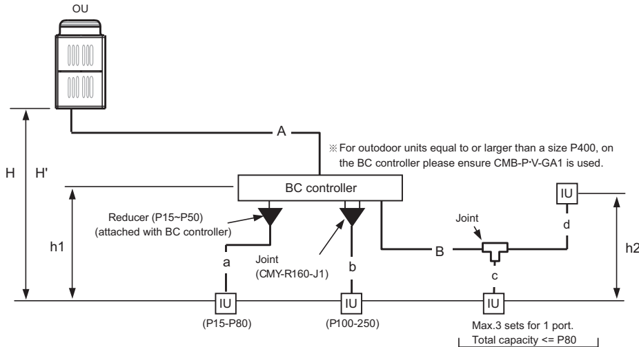
Fig. 3-1-1A Piping scheme
