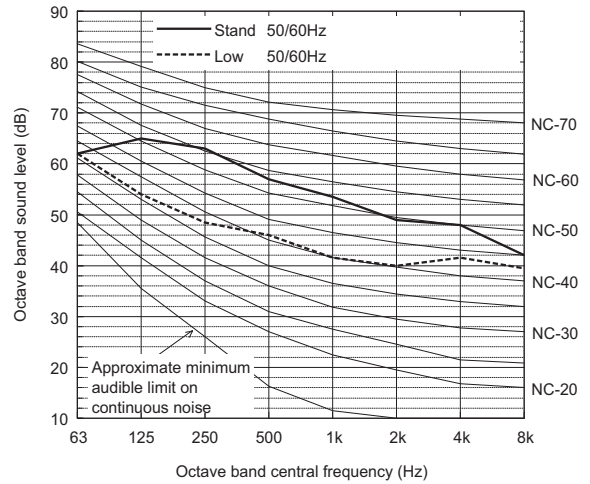
Sound level of PUHY-RP350YJM-B(-BS)
