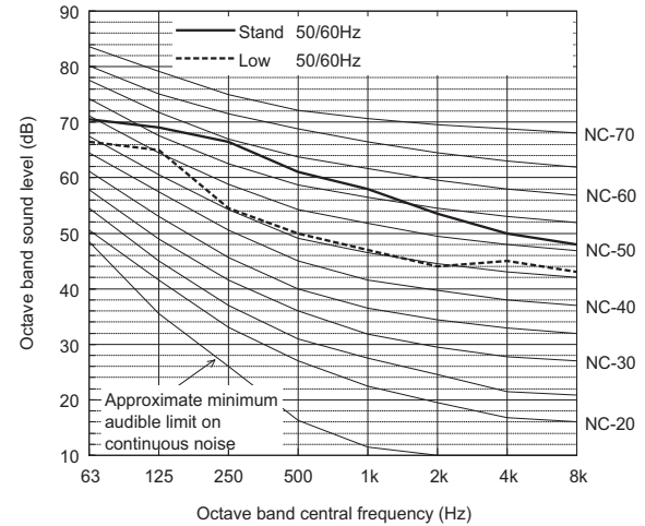
Sound level of PUHY-RP900YSJM-B(-BS)
