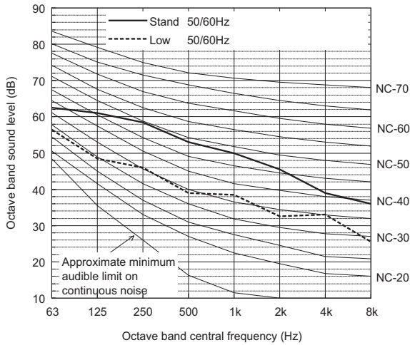
Sound level of PUHY-RP200YJM-B(-BS)
