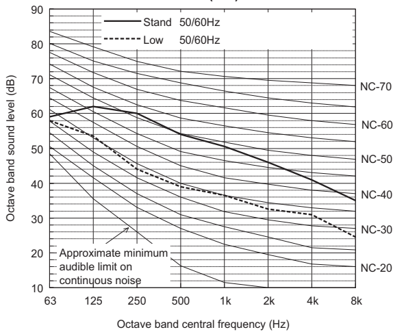
Sound level of PUHY-RP250YJM-B(-BS)
