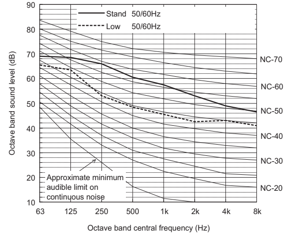
Sound level of PUHY-RP850YSJM-B(-BS)
