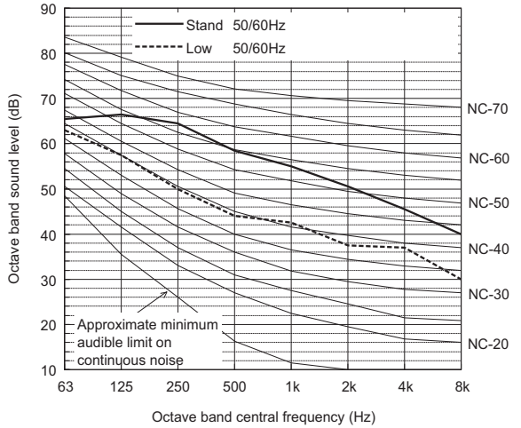
Sound level of PUHY-RP700YSJM-B(-BS)
