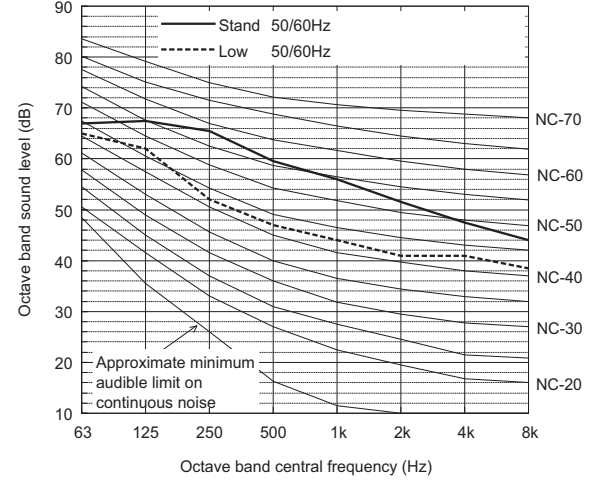
Sound level of PUHY-RP800YSJM-B(-BS)
