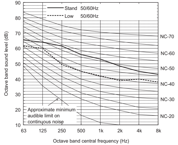
Sound level of PUHY-RP300YJM-B(-BS)
