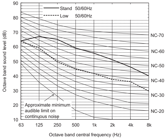
Sound level of PUHY-RP750YSJM-B(-BS)
