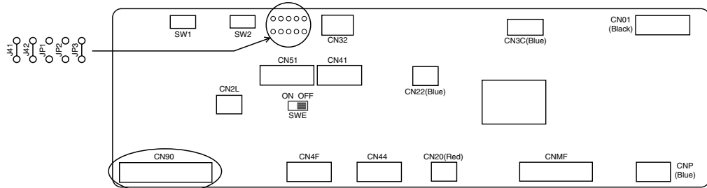
CN90: Connector for remote controller wire connection Controller circuit board on the indoor unit (reference)
