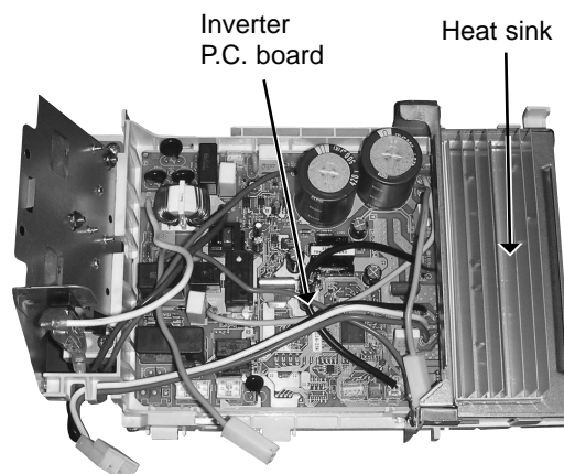
Photo 4 (Inverter assembly)
