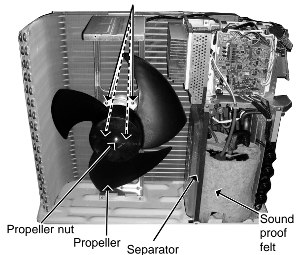
Screws of the outdoor fan motor
