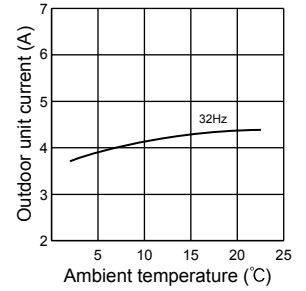
60-class unit
