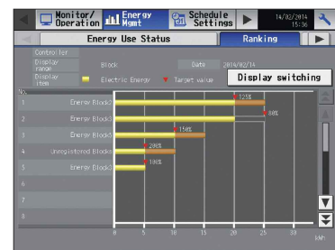
Indoor Unit Energy Consumption Ranking Screen
