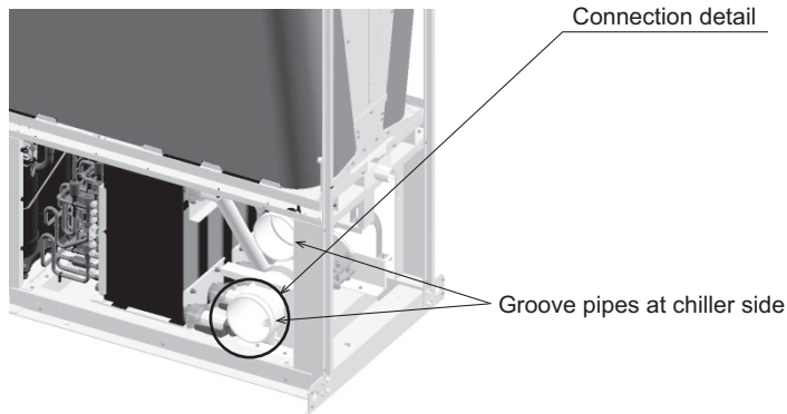
150A housing type joint
