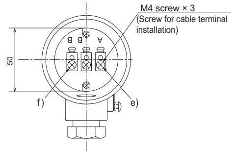
Terminal block on the sensor
