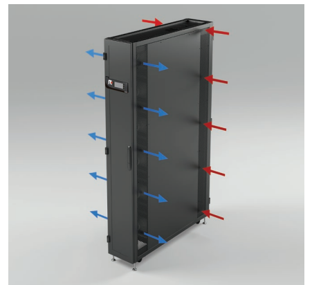
Frontal air delivery from both sides. Rear air suction from both sides.
