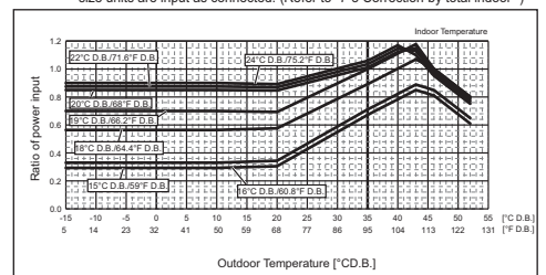
Fig.2-2 Outdoor unit temperature correction (power input) *3
