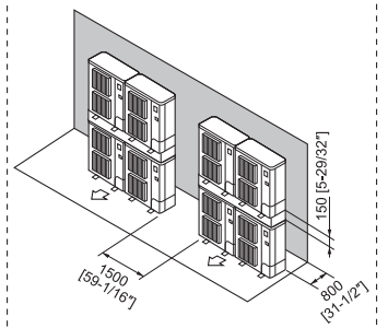
Fig. 12-2-24 Parallel individuals arrangement
