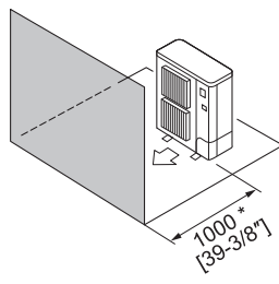
Fig. 12-2-18 Obstacles at front only
