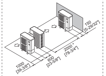
Fig. 12-2-24 Parallel individuals arrangement
