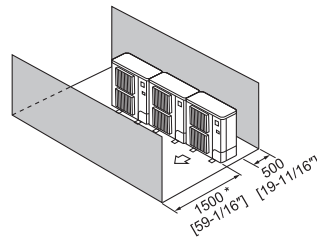
Fig. 12-2-23 Obstacles at front and rear only
