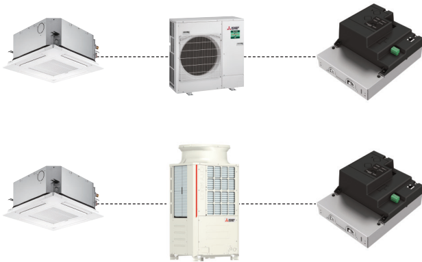
System Diagram MCC-50E
