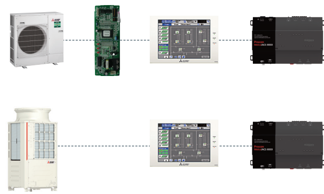
System Diagram MELCOJACE-8000
