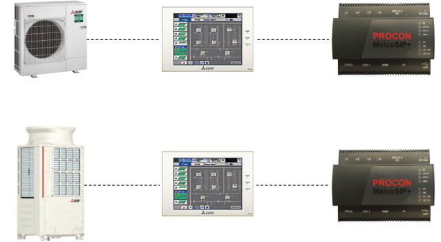
System Diagram MELCOBEMS SIP+
