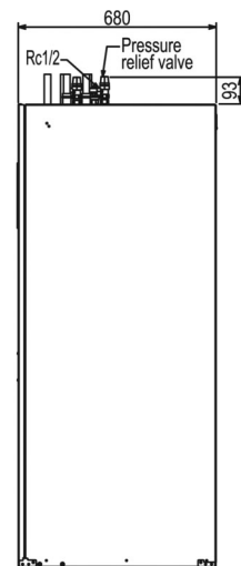
Right View Rear View
