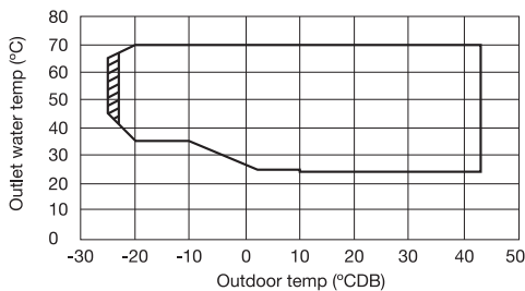
Outdoor temp. -25°CDB/Outlet water temp. 45-65°C Outdoor temp. -20°CDB/Outlet water temp. 35-70°C Outdoor temp. 43°CDB/Outlet water temp. 24-70°C
