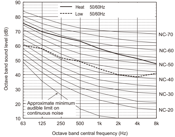
Sound level of PUHY-P300YNW-A2(-BS)
