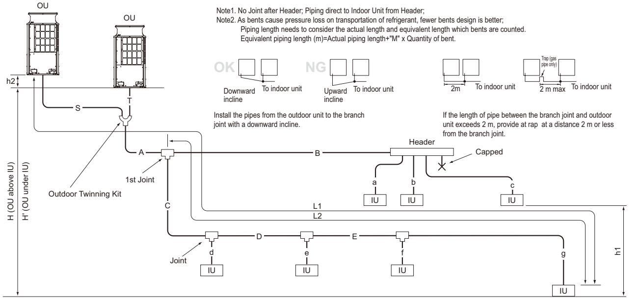
Fig. 12-2-2A Piping scheme
