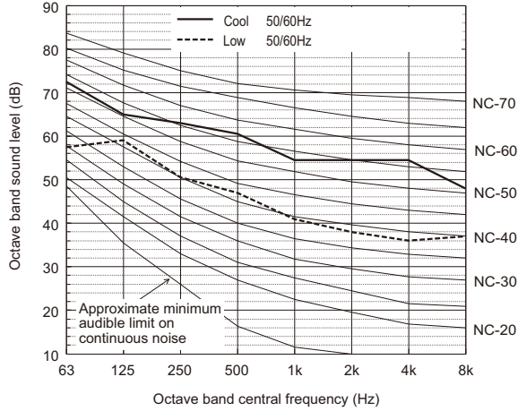
Sound level of PUHY-P500YSNW-A2(-BS)
