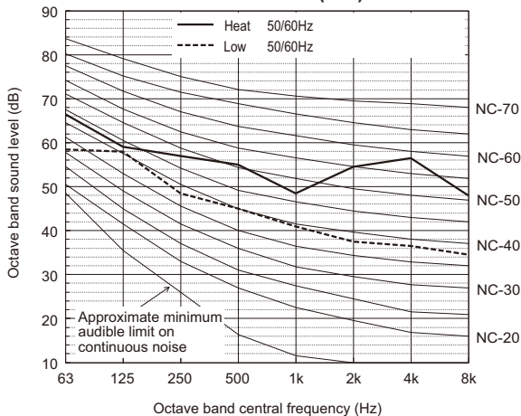
Sound level of PUHY-P250YNW-A2(-BS)
