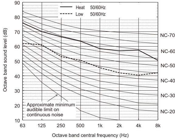
Sound level of PUHY-P550YSNW-A2(-BS)
