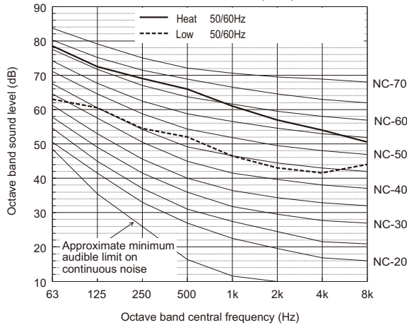
Sound level of PUHY-P600YSNW-A2(-BS)
