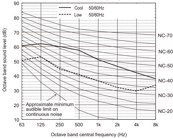
Sound level of PUHY-P200YNW-A2(-BS)
