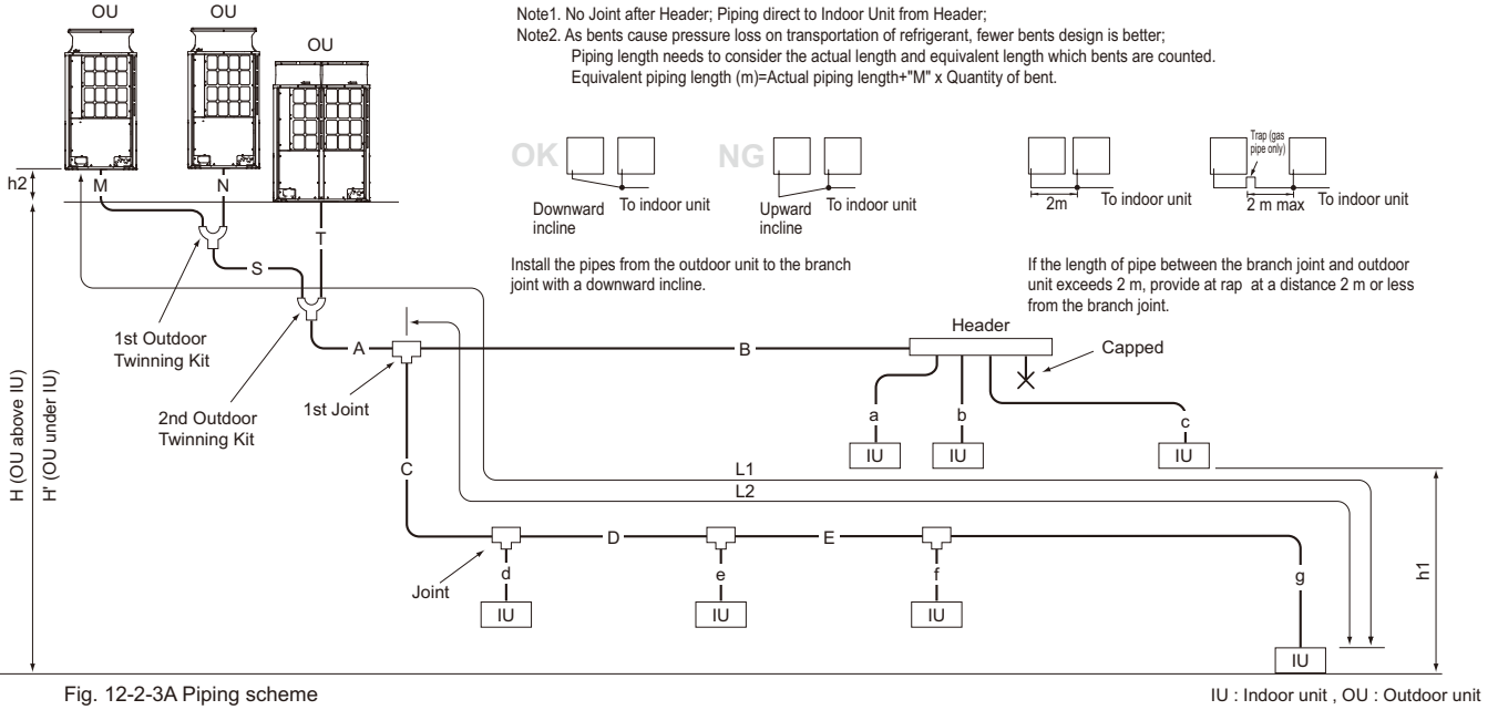
Fig. 12-2-3A Piping scheme
