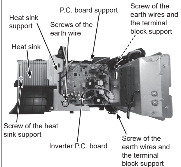
Photo 4 (Inverter assembly)
