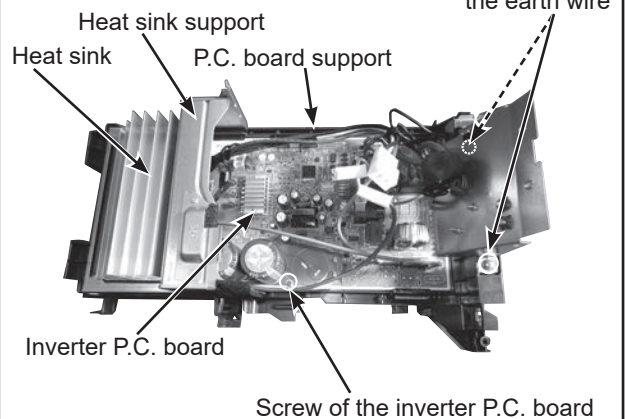
Photo 6 (Inverter assembly)
