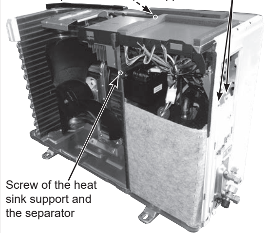
Photo 6 (Inverter assembly)
