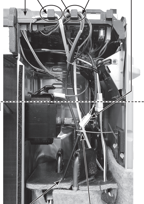
Pass the lead wire of compressor protector through the top felt hole.
