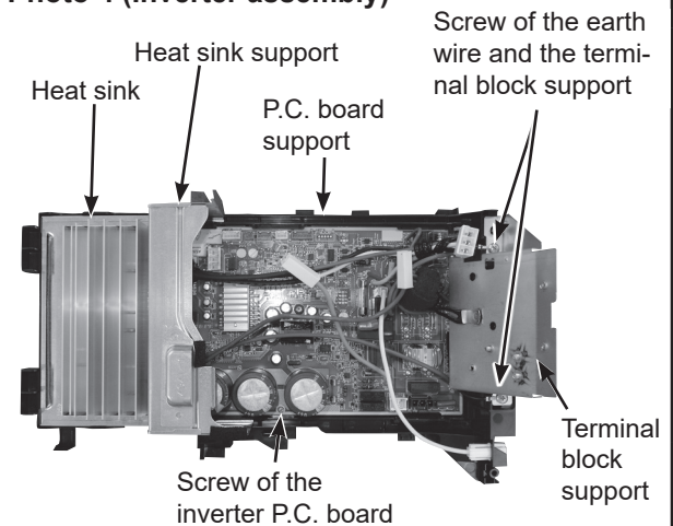
Photo 4 (Inverter assembly)
