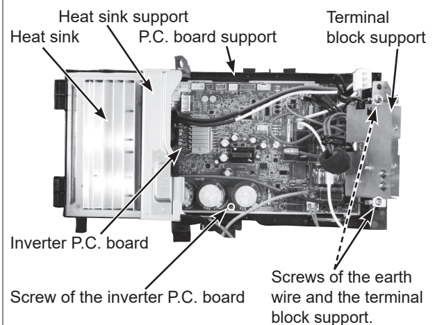
Photo 5 (Inverter assembly)
