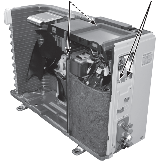
Photo 4 (Inverter assembly)
