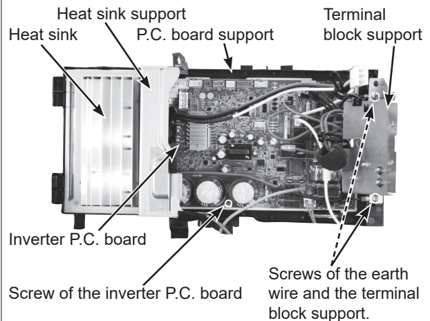
Photo 4 (Inverter assembly)
