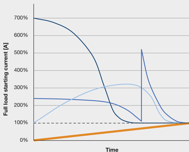
In-rush currents
