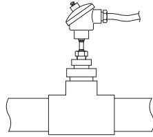
Vertical installation
