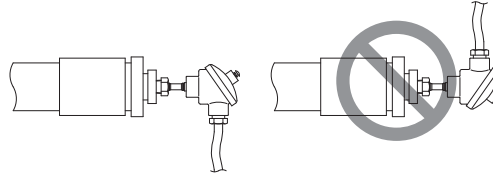
Horizontal installation
