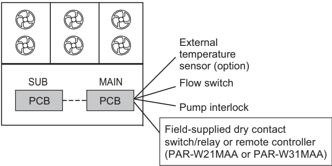
(2) Multiple module connection system (2-6 modules)
