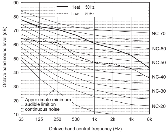
Sound level of PURY-EM800YSXM-A
