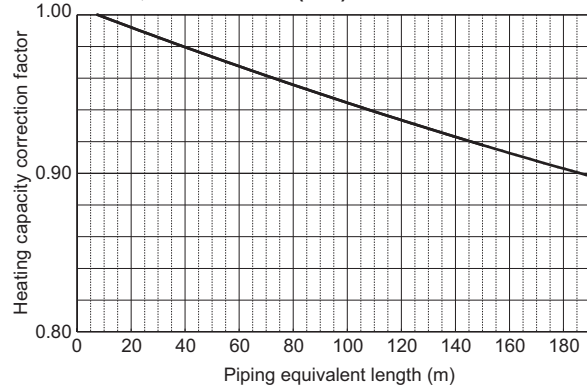
PURY-EM250, 300YXM-A/TR (-BS)
