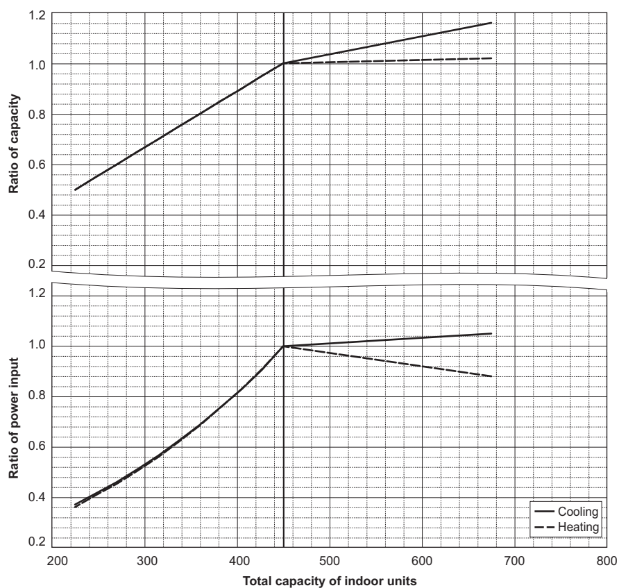
PURY-EM450YSXM-A/TR
