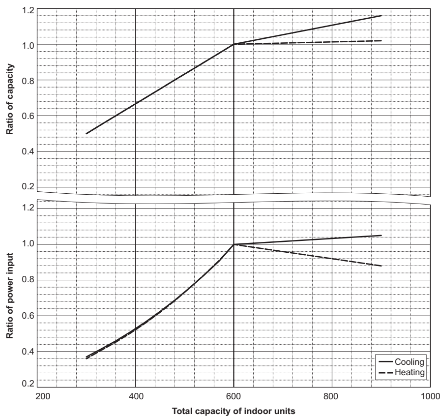
PURY-EM650YSXM-A/TR
