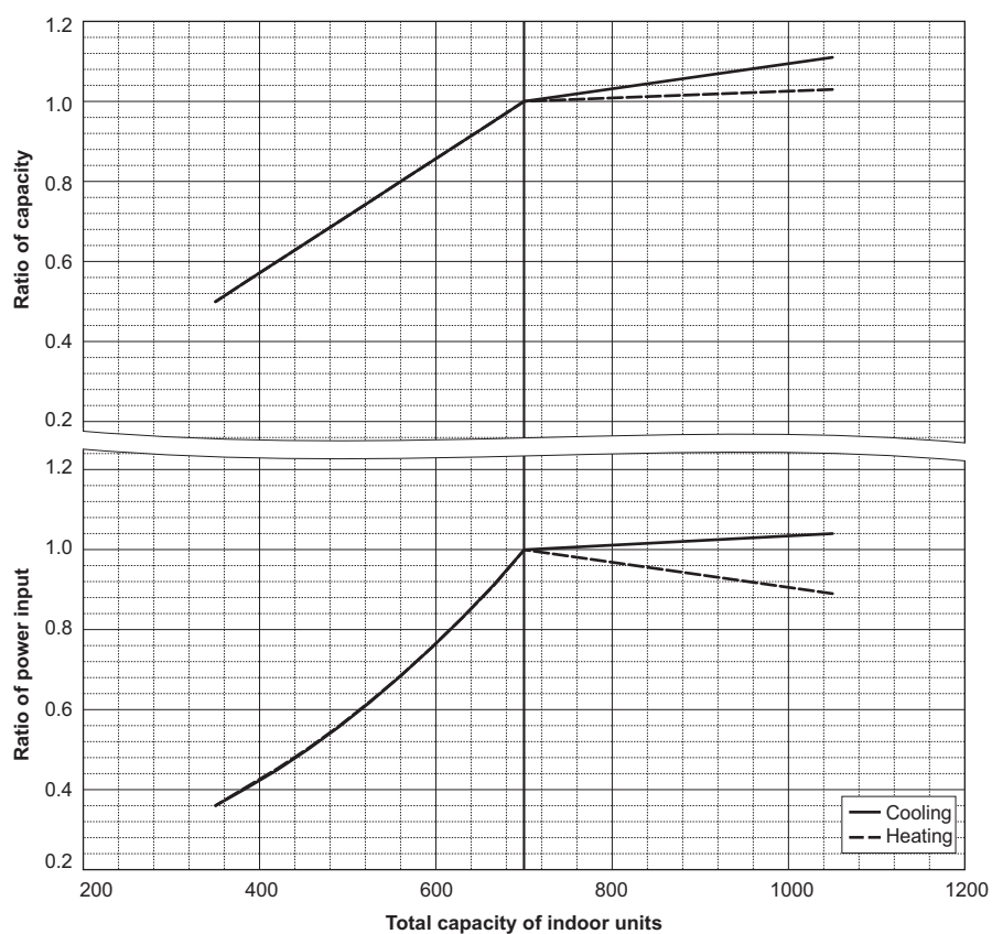
PURY-EM750YSXM-A/TR
