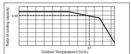
Fig.2 Outdoor unit temperature correction To be used to correct outdoor unit only
