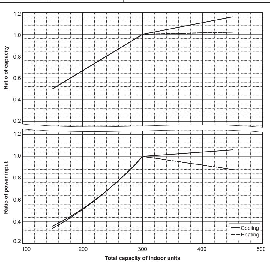
PURY-EM350YXM-A/TR
