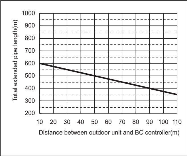
[PURY-EM350, 400, 450, 500YXM-A/TR]
