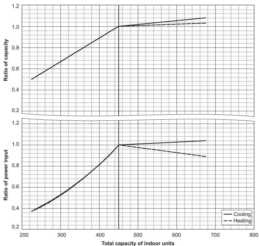
PURY-EM450YXM-A/TR
