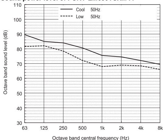
Sound power level of PURY-EM650YSXM-A
