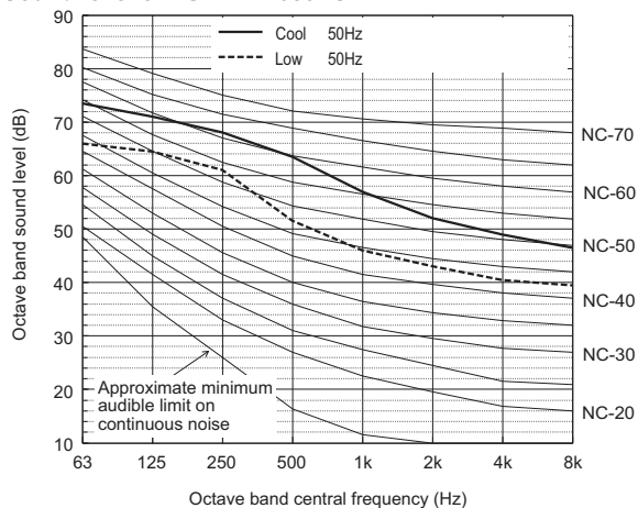
Sound level of PURY-EM850YSXM-A
