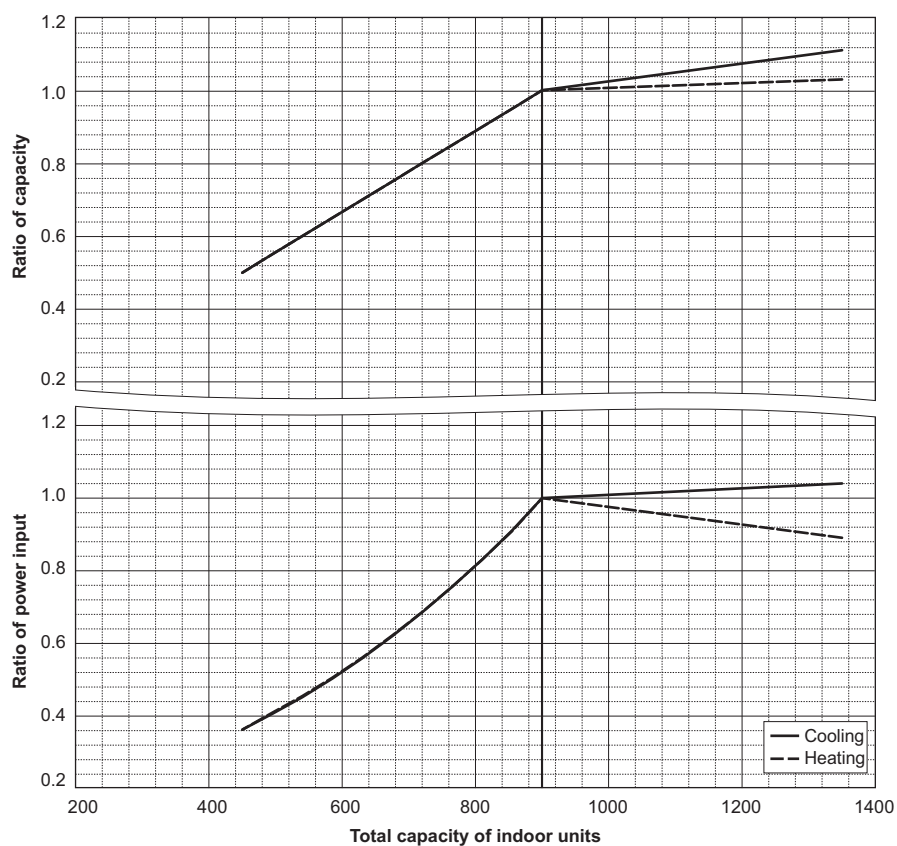
PURY-EM950YSXM-A/TR
