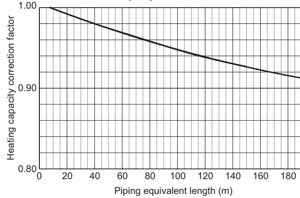
PURY-EM350YXM-A/TR (-BS)
