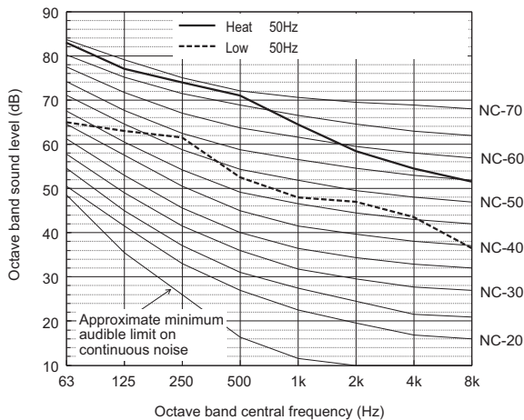
Sound level of PURY-EM900YSXM-A
