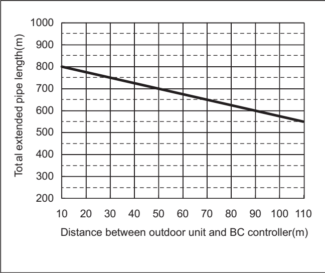
[PURY-EM650YSXM-A/TR]
