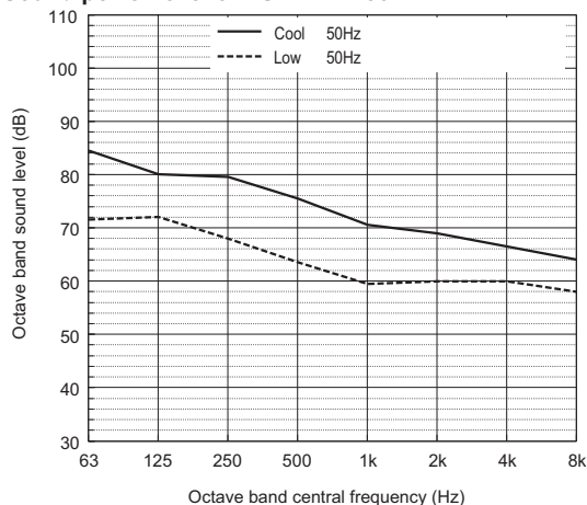
Sound power level of PURY-EM250YXM-A
