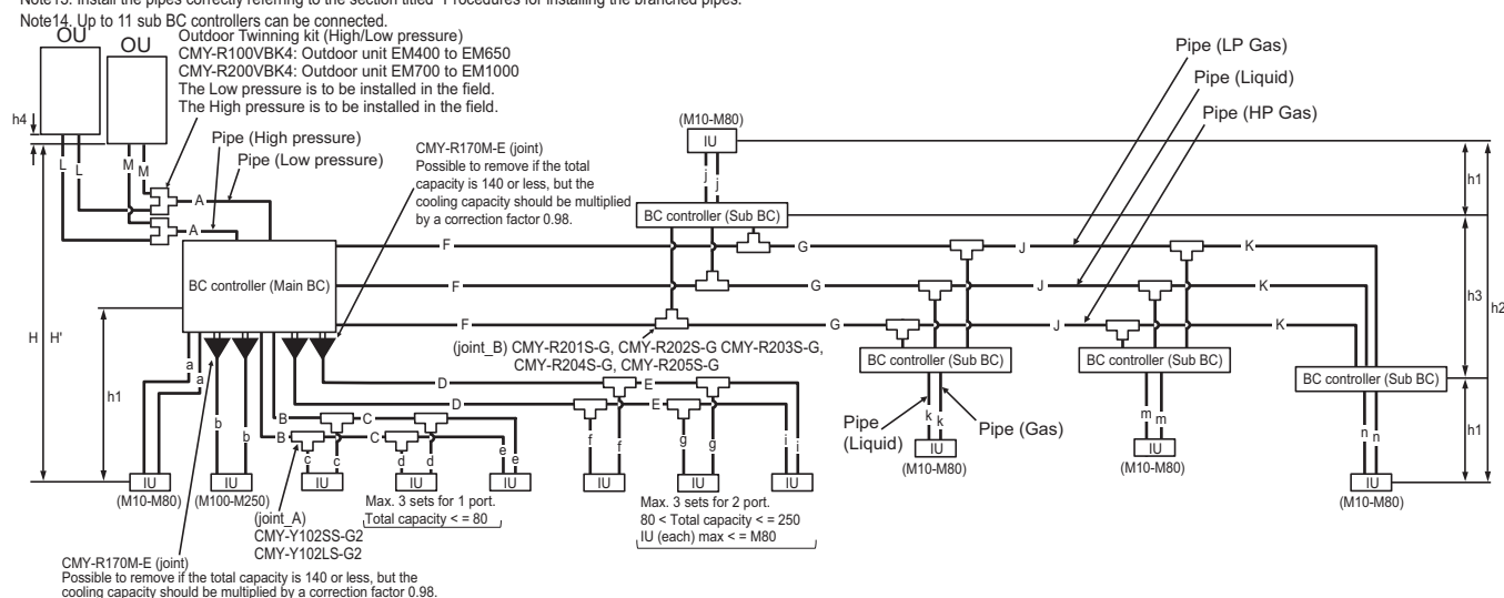
Fig. Piping scheme
