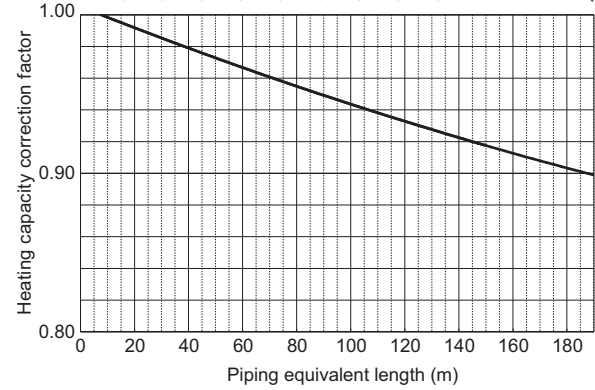
PURY-EM550, 600, 650, 700, 750, 800, 850, 900, 950, 1000YXM-A/TR (-BS)
