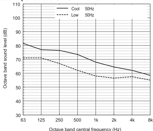
Sound power level of PURY-EM200YXM-A
