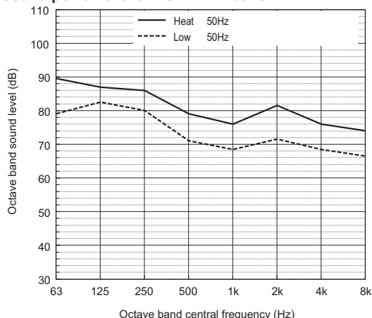
Sound power level of PURY-EM700YSXM-A
