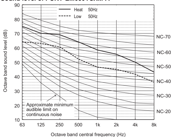
Sound level of PURY-EM650YSXM-A
