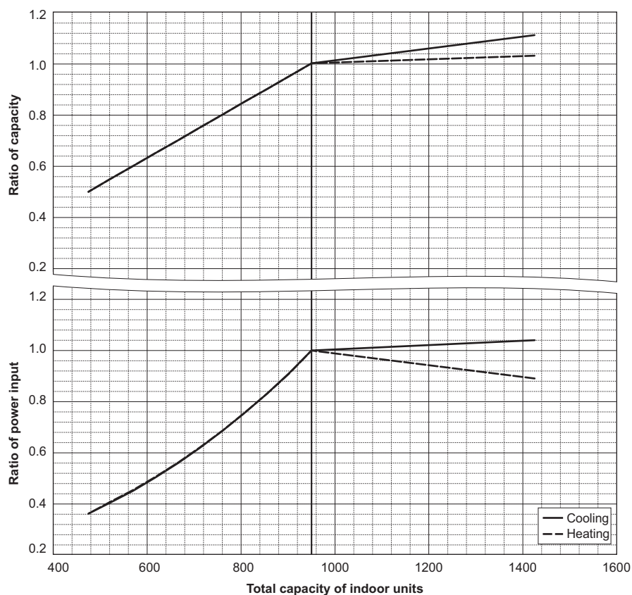
PURY-EM950YSXM-A/TR
