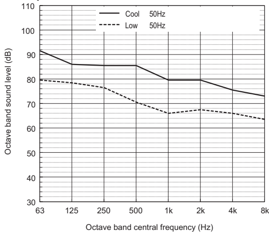
Sound power level of PURY-EM500YXM-A
