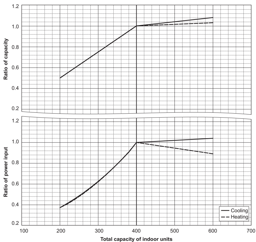
PURY-EM450YXM-A/TR
