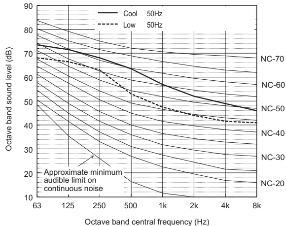
Sound level of PURY-EM800YSXM-A
