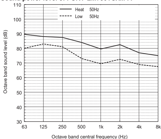
Sound power level of PURY-EM750YSXM-A
