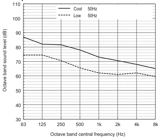
Sound power level of PURY-EM450YSXM-A
