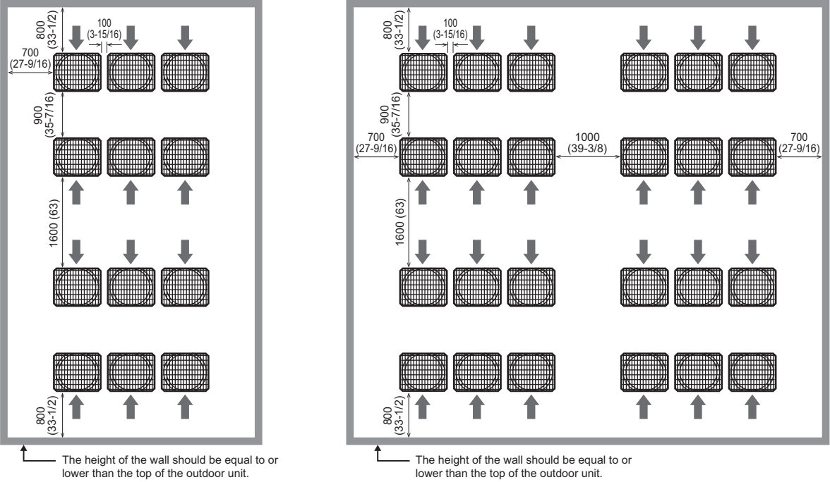
(4) Example of installation in a walled-in area (on all four sides *1)
