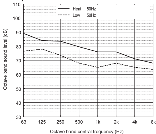
Sound power level of PURY-EM300YXM-A
