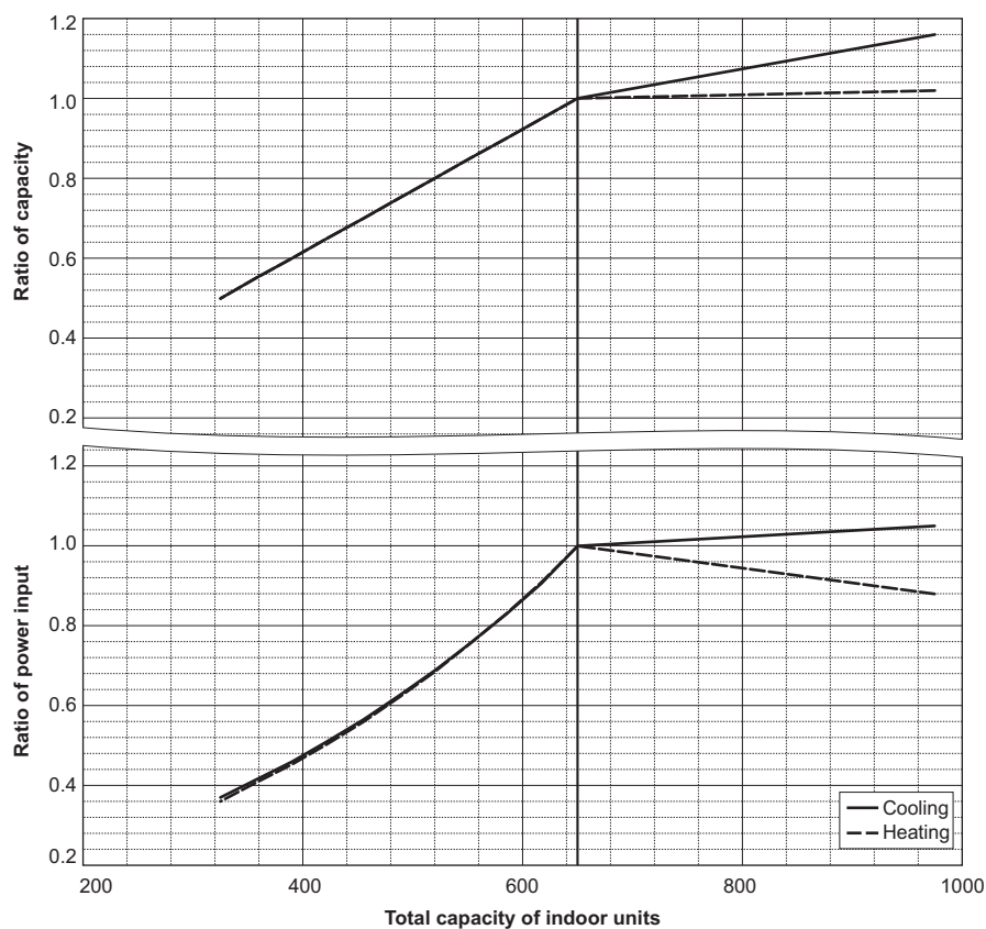
PURY-EM650YSXM-A/TR
