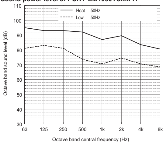
Sound power level of PURY-EM1000YSXM-A
