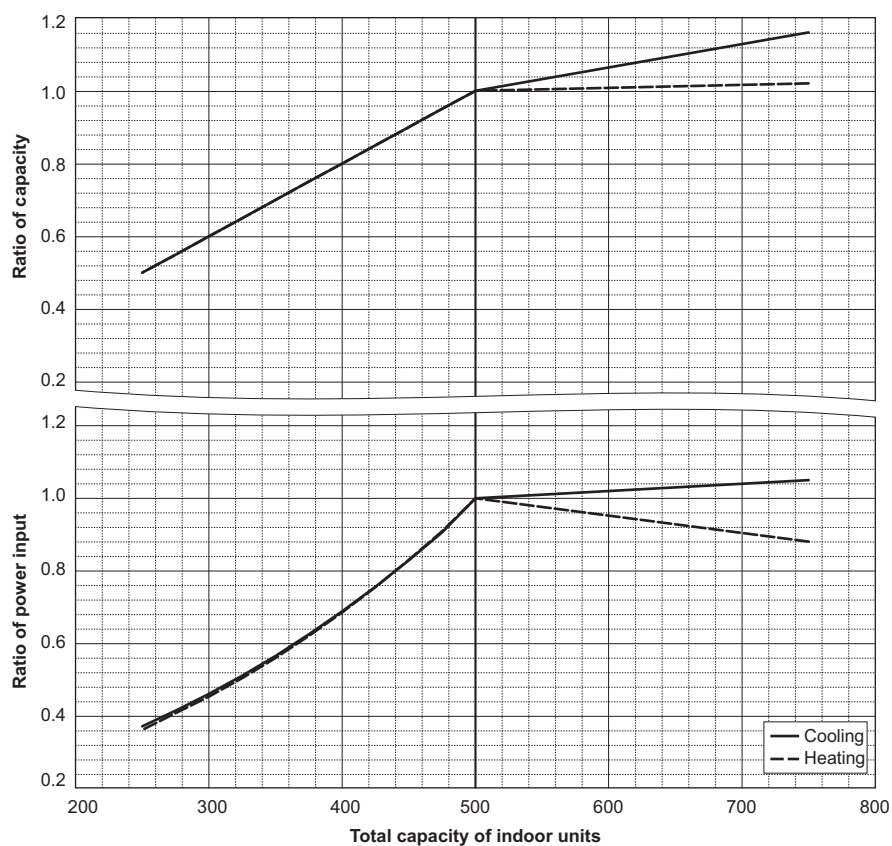
PURY-EM550YSXM-A/TR
