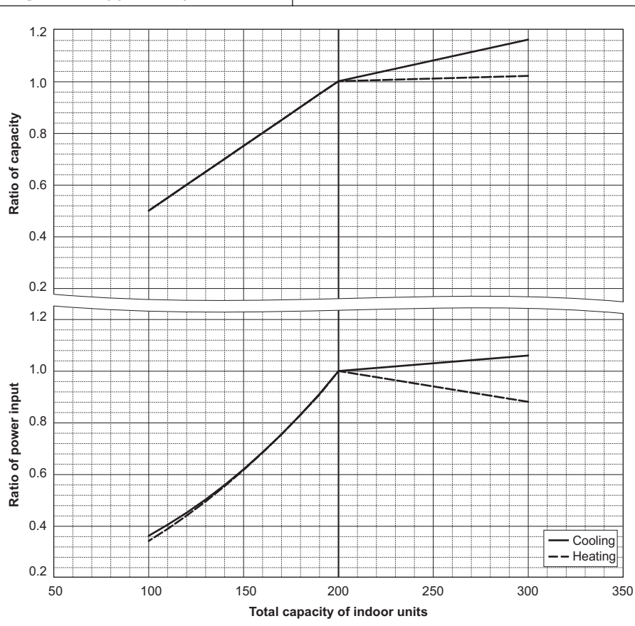
PURY-EM250YXM-A/TR
