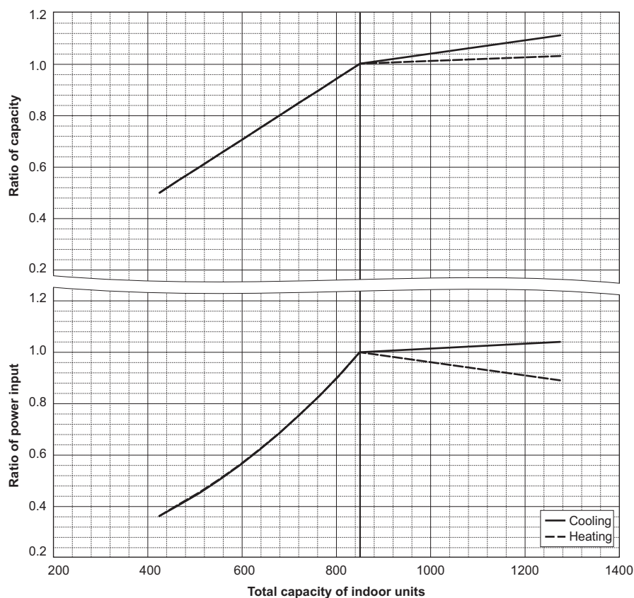
PURY-EM850YSXM-A/TR
