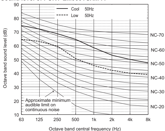
Sound level of PURY-EM900YSXM-A
