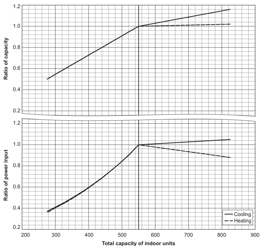
PURY-EM550YSXM-A/TR
