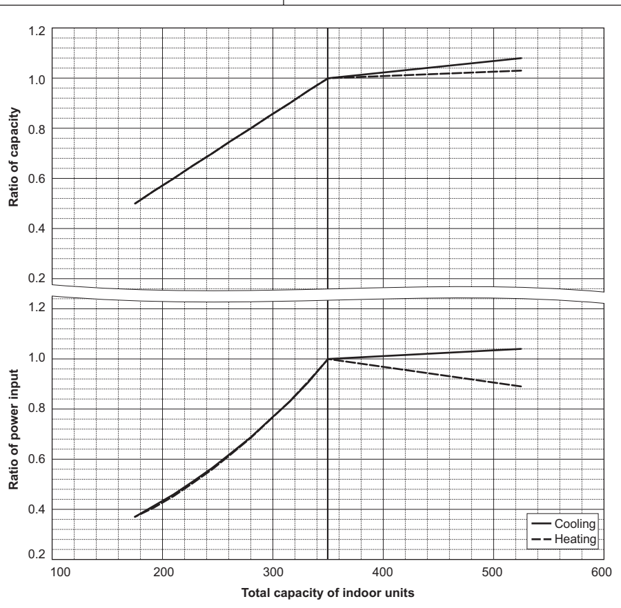
PURY-EM350YXM-A/TR
