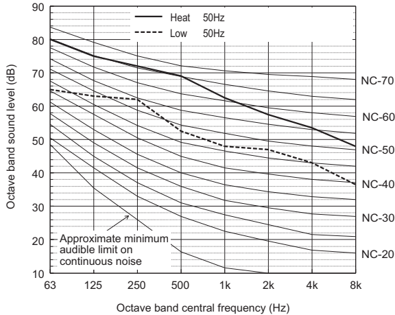
Sound level of PURY-EM850YSXM-A
