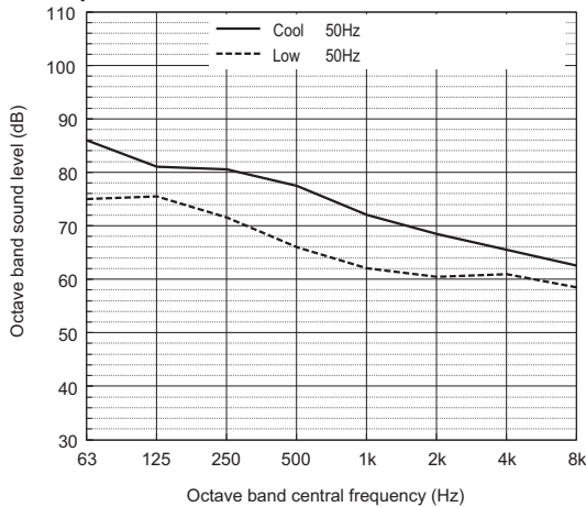
Sound power level of PURY-EM400YSXM-A
