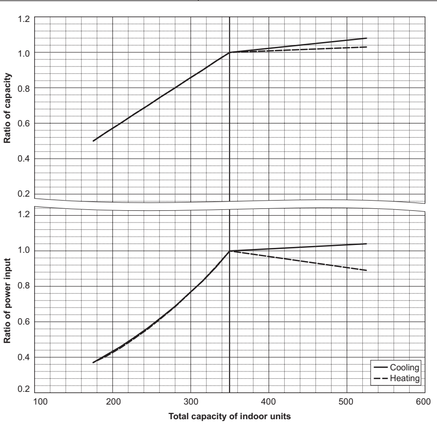
PURY-M350XMA-A
