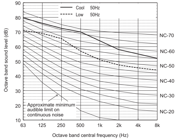
Sound level of PURY-M1000YSXM-A
