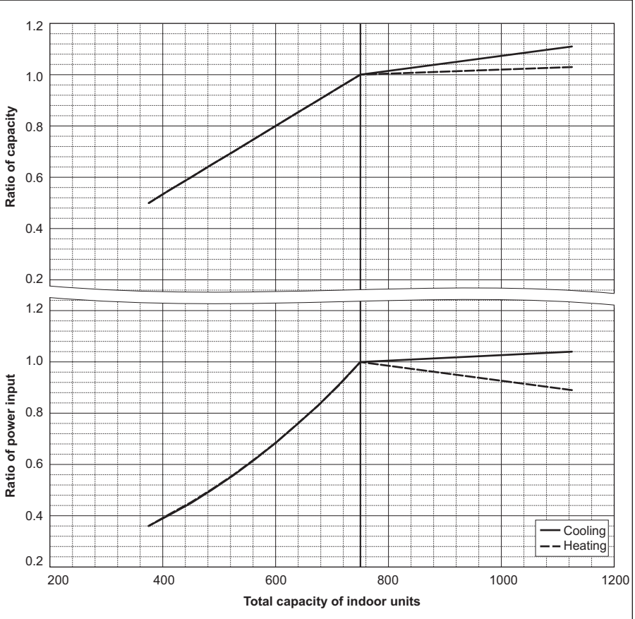
PURY-M750YSXM-A
