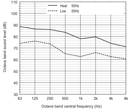
Sound power level of PURY-M400YXM-A
