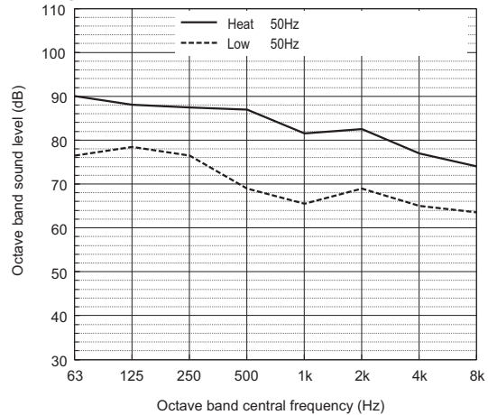
Sound power level of PURY-M450YXM-A
