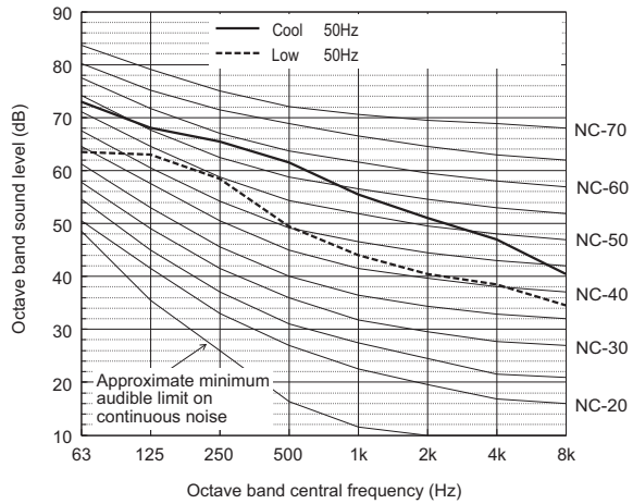
Sound level of PURY-M650YSXM-A
