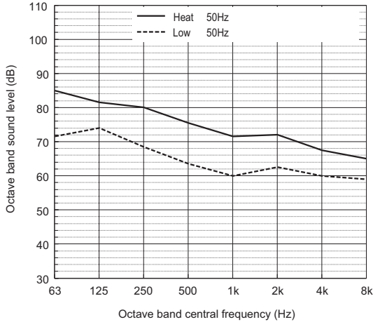
Sound power level of PURY-M250YXM-A
