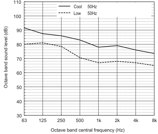
Sound power level of PURY-M800YSXM-A
