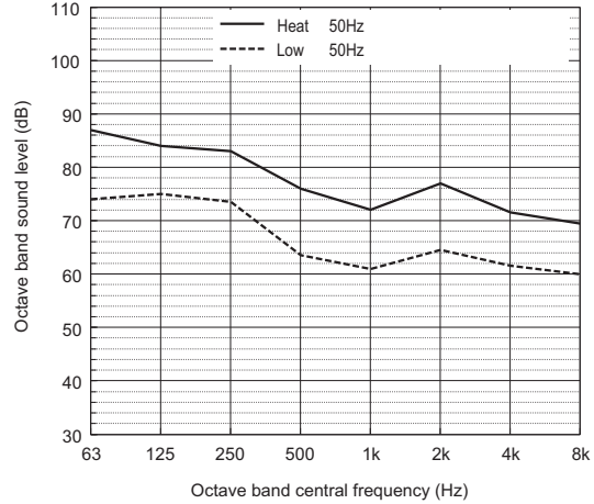
Sound power level of PURY-M350YXM-A
