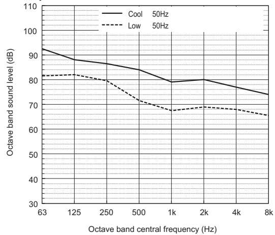
Sound power level of PURY-M900YSXM-A
