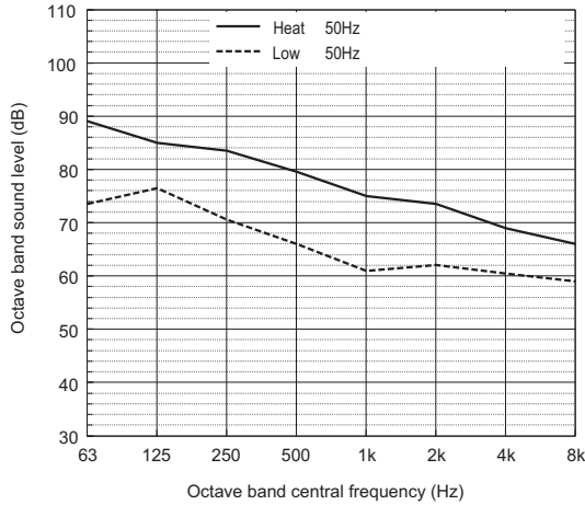
Sound power level of PURY-M400YSXM-A
