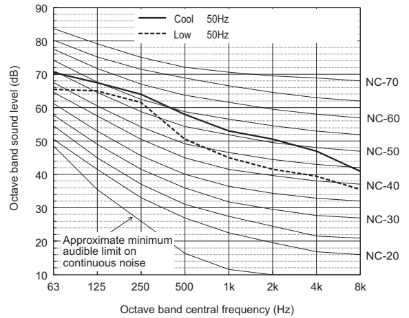
Sound level of PURY-M700YSXM-A
