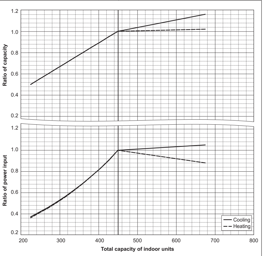
PURY-M450YSXM-A
