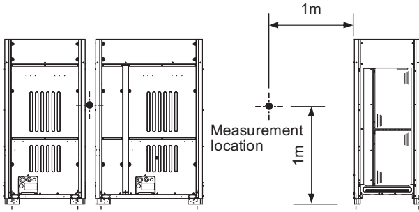
Measurement condition PURY-M650YSXM-A(-BS)
