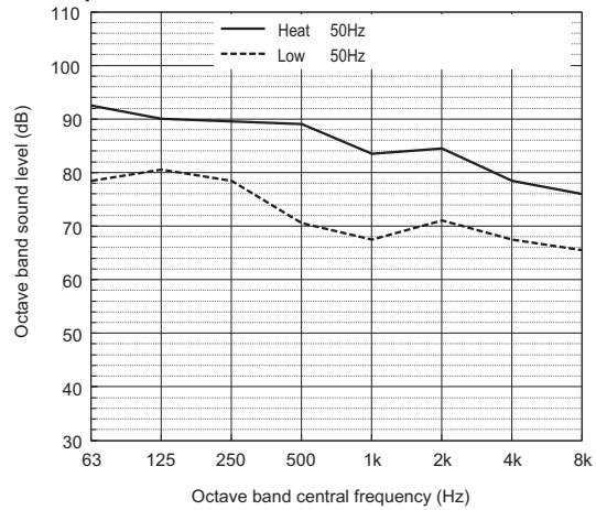
Sound power level of PURY-M850YSXM-A
