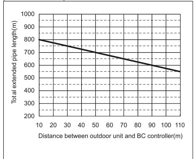
[PURY-M650YSXM-A]
