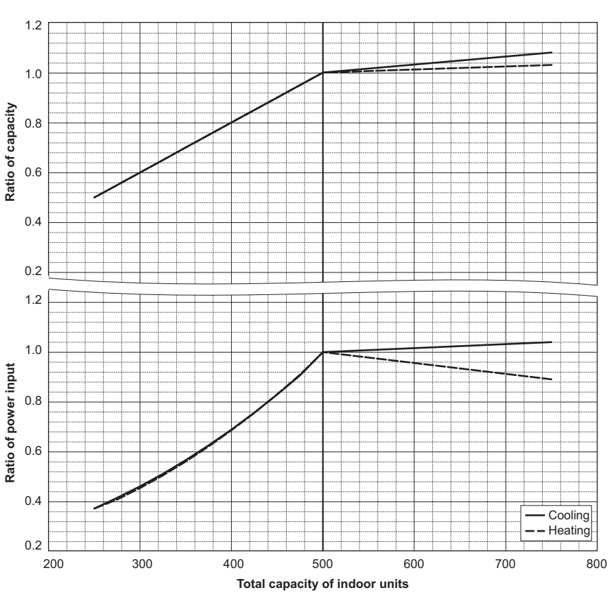
PURY-M500YXM-A
