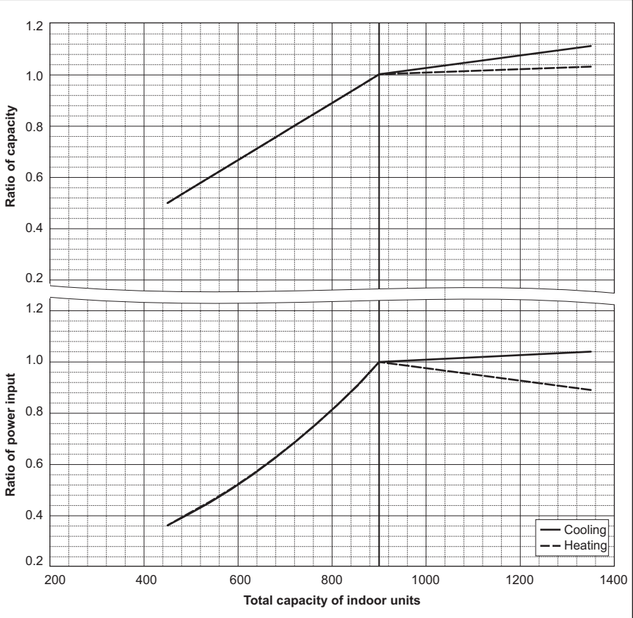
PURY-M950YSXM-A
