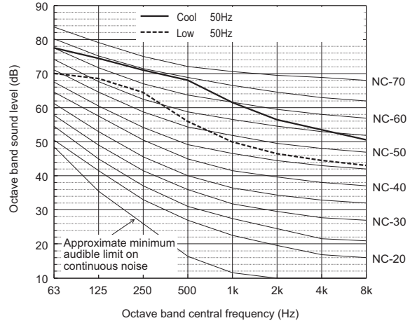
Sound level of PURY-M950YSXM-A
