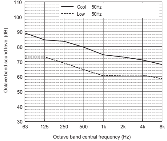
Sound power level of PURY-M500YSXM-A
