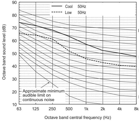
Sound level of PURY-M800YSXM-A
