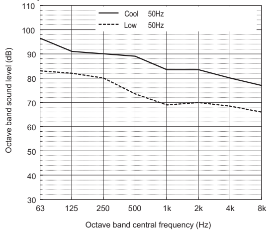
Sound power level of PURY-M1000YSXM-A
