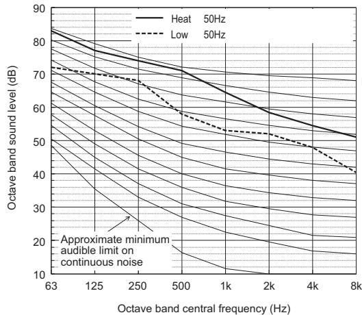
Sound level of PURY-M900YSXM-A
