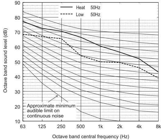
Sound level of PURY-M800YSXM-A
