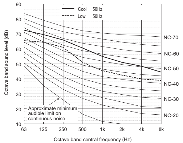
Sound level of PURY-M750YSXM-A
