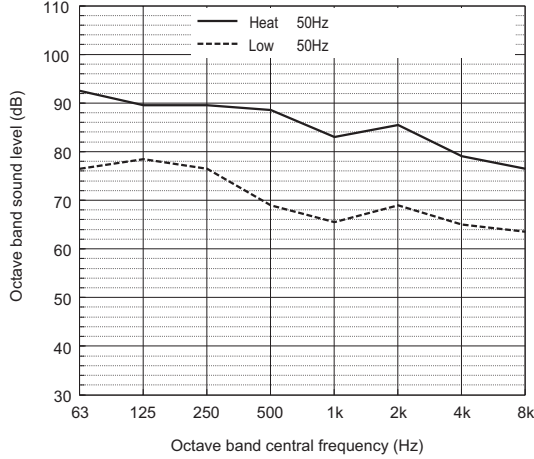
Sound power level of PURY-M500YXM-A
