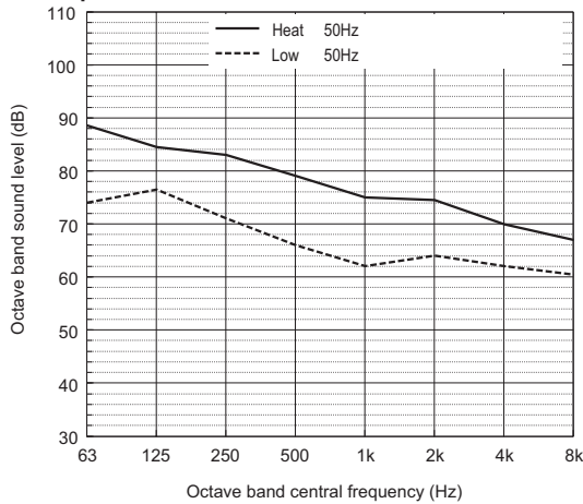
Sound power level of PURY-M450YSXM-A
