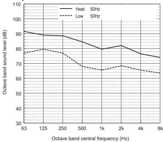
Sound power level of PURY-M750YSXM-A
