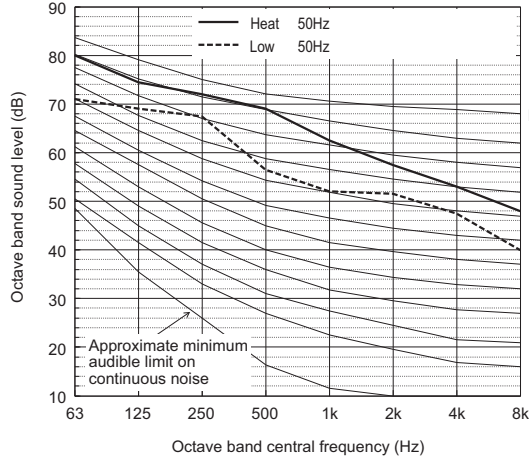
Sound level of PURY-M850YSXM-A
