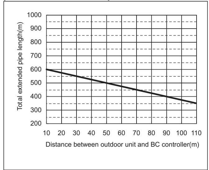
[PURY-M350, 400, 450, 500YXM-A]
