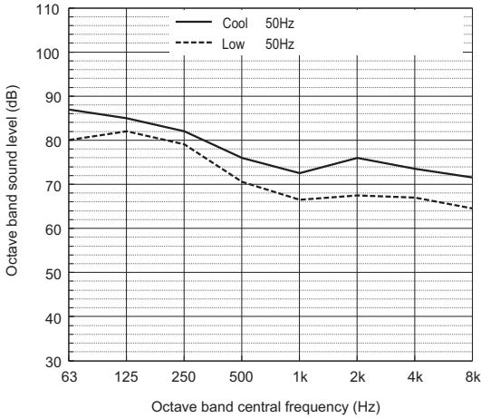
Sound power level of PURY-M700YSXM-A
