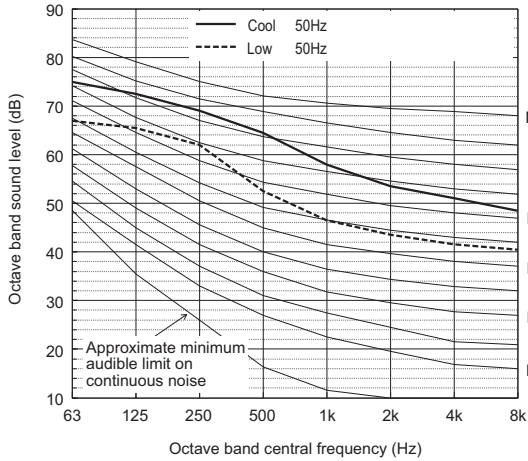
Sound level of PURY-M850YSXM-A
