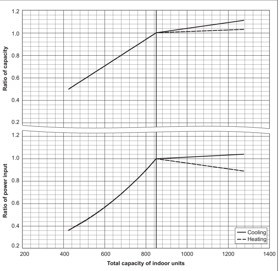
PURY-M850YSXM-A
