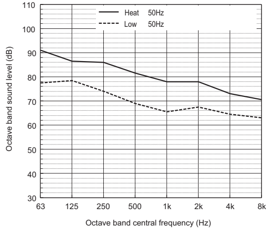
Sound power level of PURY-M550YSXM-A
