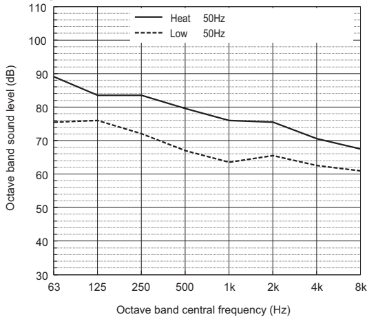
Sound power level of PURY-M300YXM-A
