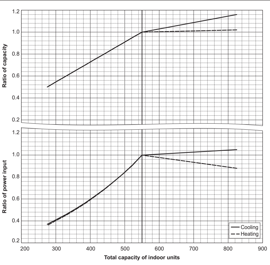
PURY-M550YSXM-A
