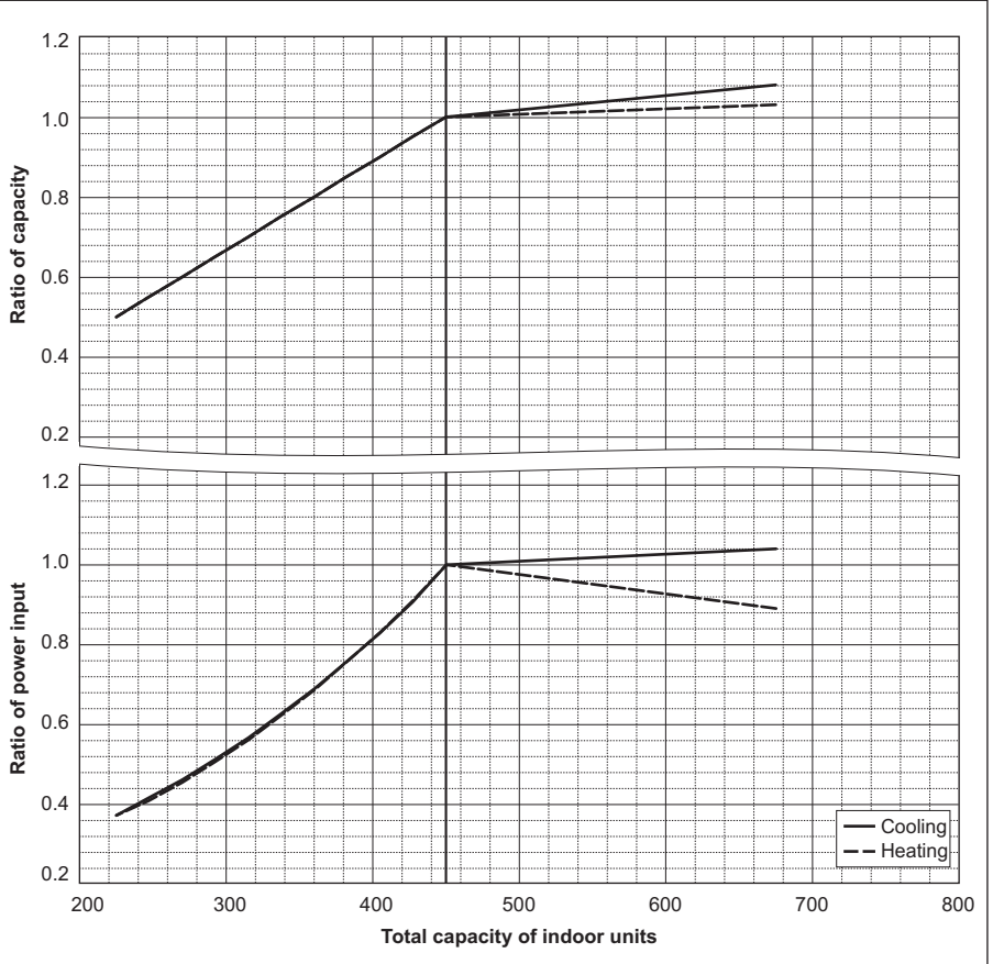
PURY-M450YXM-A
