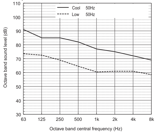
Sound power level of PURY-M600YSXM-A
