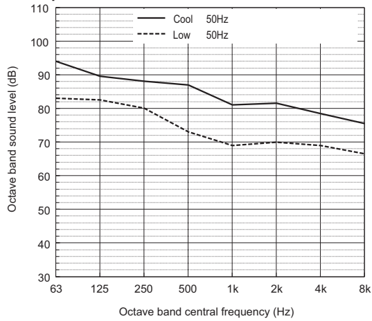
Sound power level of PURY-M950YSXM-A
