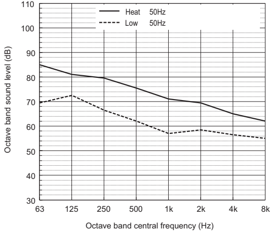
Sound power level of PURY-M200YXM-A
