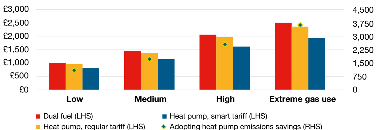
Figure 4: Household bills by consumption tier across policy options with estimated emissions savings from switching to a heat pump 30
