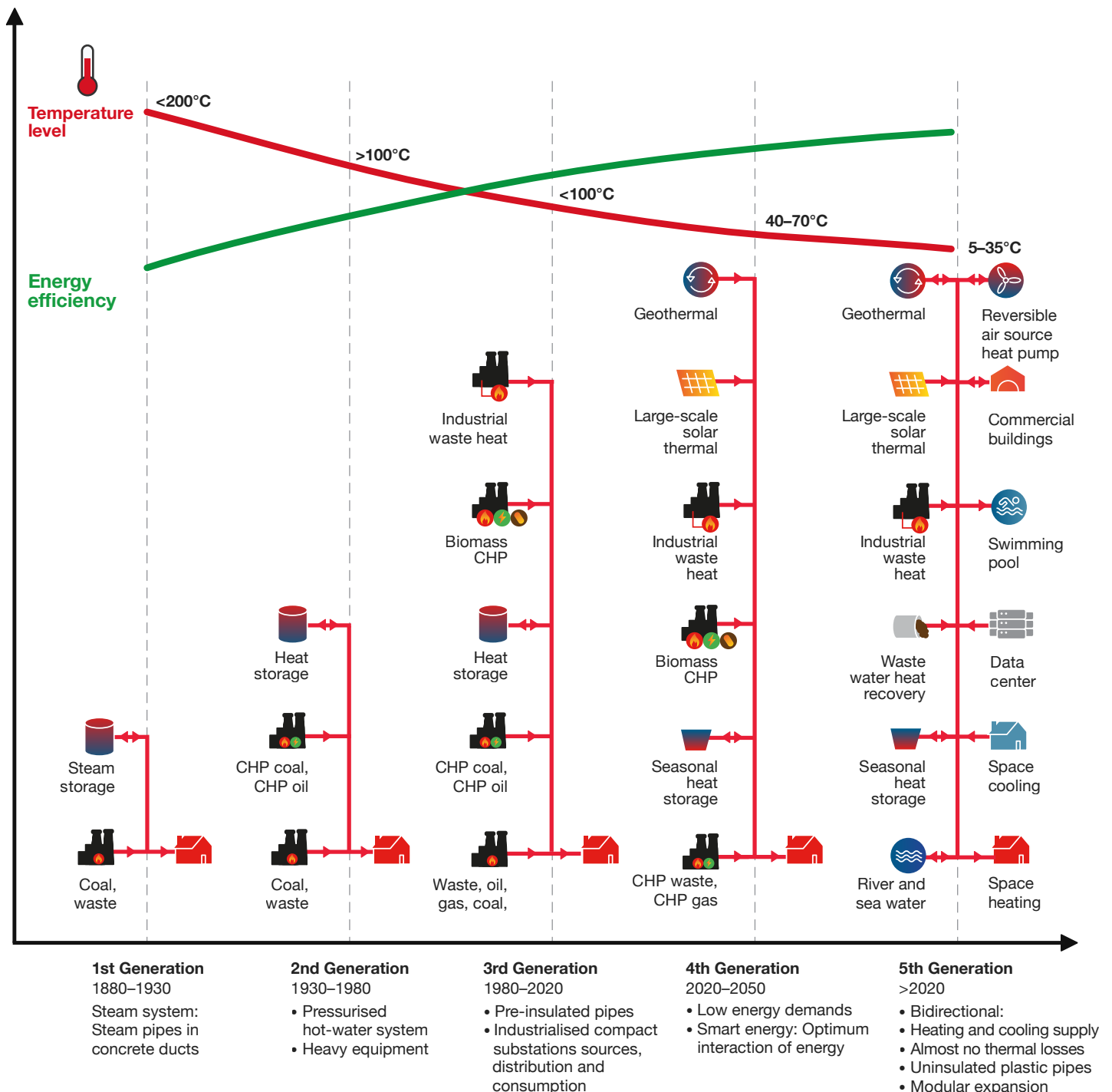
Appendix figure 3: Visualisation of the evolution of district heating and cooling networks, from the first to the fifth generation of DHC networks. 53
